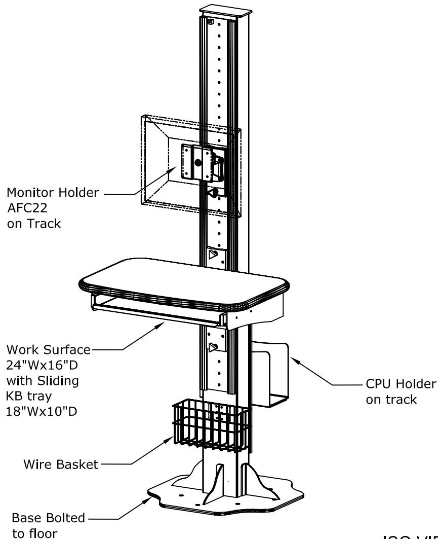
ISO VIEW
